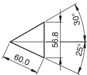
Cam Diagram
